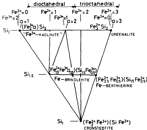
FIG. 5. Projection field for 1:1 phyllosilicates with Fe^{2+} , Fe^{3+} , and \square in octahedra.
