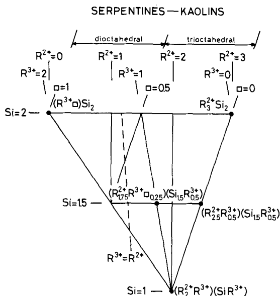
FIG. 1. Projection field for the condensed chemical composition of 1:1 phyllosilicates. Composition isolines: R^{2+} —Mg, Fe 2+ , Ni, Mn, Zn; R^{3+} —Al, Fe 3+ , Cr; □—vacancies.
