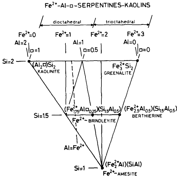
FIG. 4. Projection field for 1:1 phyllosilicates with Fe^{2+} , Al and \square in octahedra.
