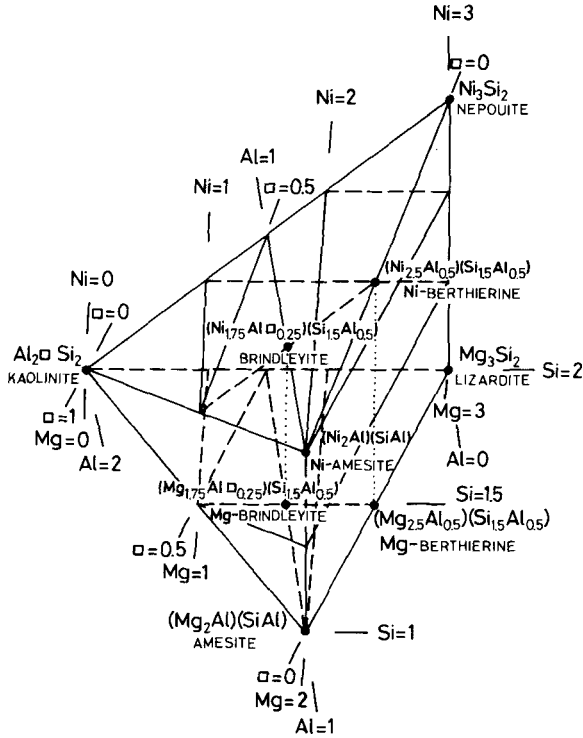
FIG. 2. Composition polyhedron for 1:1 phyllosilicates with Mg, Fe 2+ , Al and □ in octahedra.
