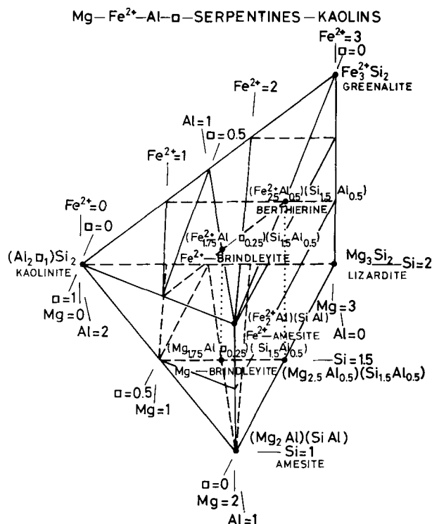
FIG. 6. Composition polyhedron for 1:1 phyllosilicates with Mg, Ni, Al, and □ in octahedra.
