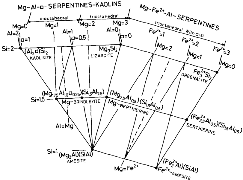
FIG. 3. Projection field for phyllosilicates with Mg, Al and □, (a bottom) and with Mg, Fe 2+ and Al (a side wall of Fig. 2).
