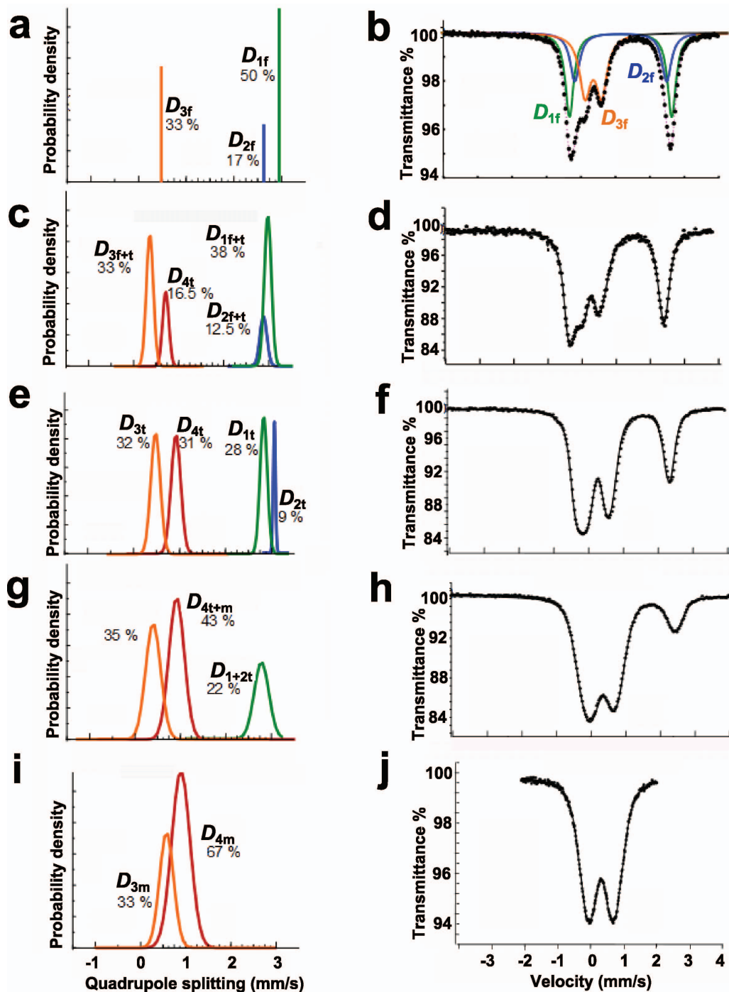
FIG. 7. Mössbauer spectra measured at 78 K of synthetic green rust samples for values of x = [\text{Fe}^{3+}]/[\text{Fe}_{10d}] in the range 1/2 –1. (a) Probability density for Gaussian distributions of quadrupole splittings fitted using Voigt-function profiles, and (b) total spectrum showing fitted doublets for x = 1/2 ; (c) and (d) are corresponding data for x = 1/2 ; (e) and (f) for x = 0.63 ; (g) and (h) for x = 0.78 ; (i) and (j) for x = 1 .
